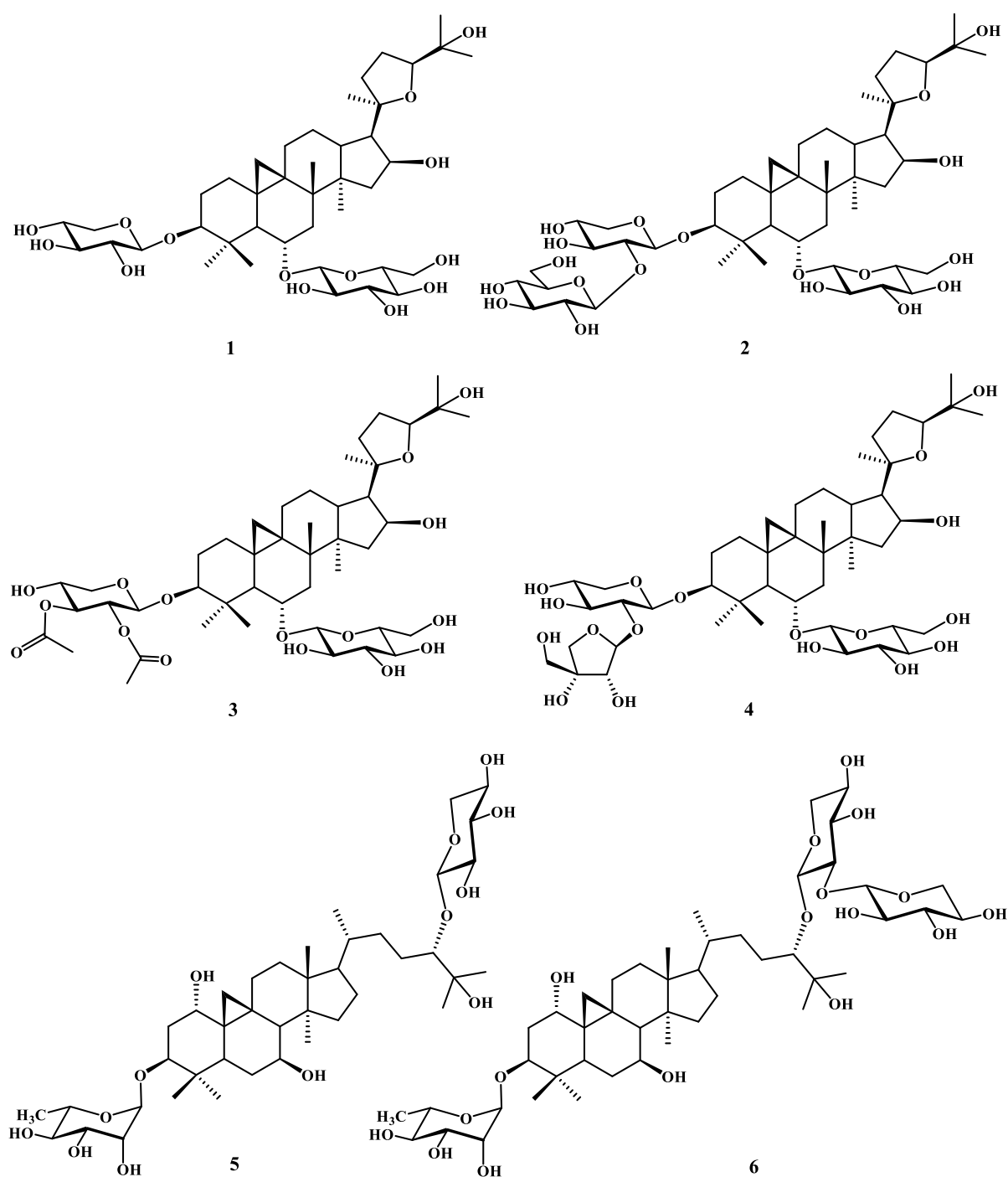
Figure 1. Structural formulae of glycosides used in the study 1: Astragaloside IV, 2: Astragaloside VI, 3: Astrasieverianin II, 4: Baibutoside, 5: Macrophyllsaponin B, 6: Macrophyllsaponin D
