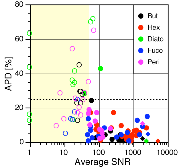
Fig. 4. HPL individual pigment APDs per sample plotted as a function of the SNR for the pigment peak. The circles and diamonds represent SeaHARRE-3 field samples and DHI Mix results, respectively. Solid circles correspond to all QA laboratories reporting a pigment is present, whereas open circles denote one or more QA laboratories not reporting a pigment is present. The yellow area highlights an average SNR of 50 or less, and the dashed line is an APD of 25% (the basic performance metric for QA results).
