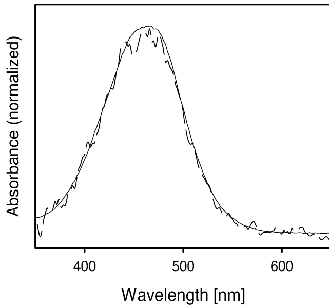
Fig. 15. In-line absorbance spectra of the Fig. 14d Pras peak with an SNR of 34 (dashed line) and a Pras standard (solid line).
