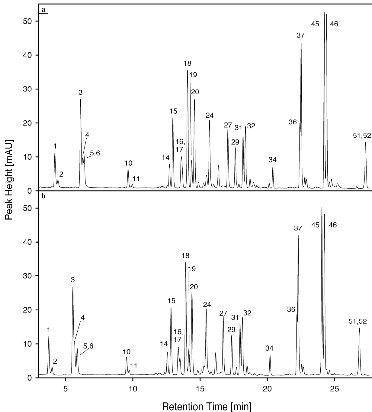
Fig. 8. Chromatograms depicting differences in separation selectivity for peaks 3–6 and 16–17 were observed from the same sample injected on two different Agilent, XDB C 8 HPLC columns: a) a newly installed column (serial number 4200), and b) a column that had been used for approximately 900 injections (S/N 4048). The peak numbers refer to pigments listed in Table 31: 1 is Chl c 3 , 2 is MVChl c 3 , 3 is Chl c 2 , 4 is MgDVP, 5 is Chl c 1 , 6 is Chlide a , 10 is Perid, 11 is Perid isomer, 14 is But, 15 is Fuco, 16 is Neo, 17 is 4k-hex-fuco, 18 is Pras, 19 is Viola, 20 is Hex, 24 is Diad, 27 is Allo, 29 is Diato, 31 is Zea, 32 is Lut, 34 is Gyroxanthin diester, 36 is DVChl b , 37 is Chl b , 45 is DVChl a , 46 is Chl a , 51 is \beta\epsilon -Car, and 52 is \beta\beta -Car.
