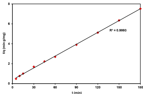
Figure 7. Plot of pseudo-second order kinetic model of BR 18 onto KF/sepiolite (pH = 8, Temperature = 20 °C).
