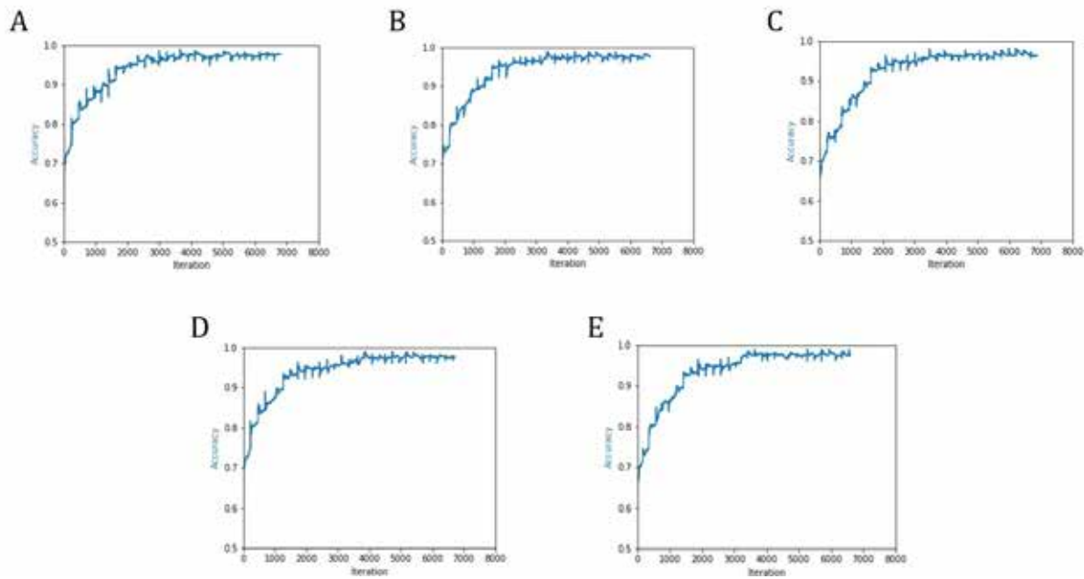
Figure 1. Accuracy of image classification during iteration. A to E represent our neural network trained with randomly divided data set. Iteration means the process of updating the model's parameter once with batch data. Accuracy refers the accuracy of image classification during iteration.
