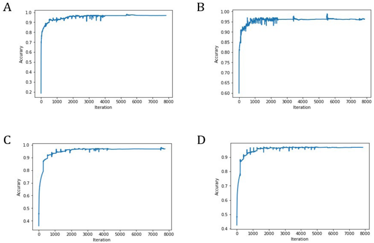
Figure 3. Accuracy of image classification during iteration using transfer learning. A to D represent our neural network trained with limited data using transfer learning. Iteration means the process of updating the model's parameter once with batch data. Accuracy refers the accuracy of image classification during iteration using transfer learning for different kinds of medical images. A, colorectal carcinoma; B, breast ductal carcinoma; C, retinal diseases; D, chest X-Ray.
