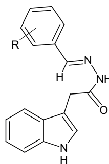
Scheme 1. Synthesized compounds
