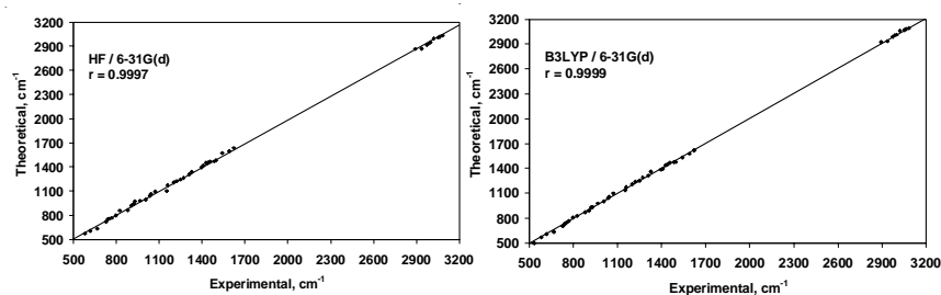
Fig. 3. Correlation graphics of calculated and experimental frequencies of title compound
