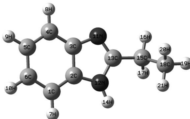
Fig. 1. Theoretical geometric structure of the 2-ethyl-1 H -benzo[ d ]imidazole
