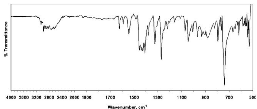
Fig. 2. FT-IR spectrum of 2-ethyl-1 H -benzo[ d ]imidazole recorded at room temperature.
